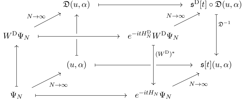
Figure 1. Diagram schematizing Theorem 1.1 and its relation with the dressed counterpart, Theorem 3.2. Each microscopic state on the front face is close to the associated mean-field state in the limit N \rightarrow \infty (lying on the face beyond), as measured by the functional \beta . The arrows are kept unlabeled if the associated map is obvious.
