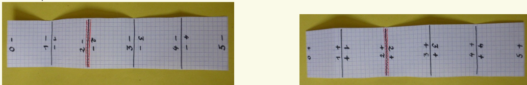
Figure 3: A tape of paper with boxes, indices on both side of borders, one face + and one face -
