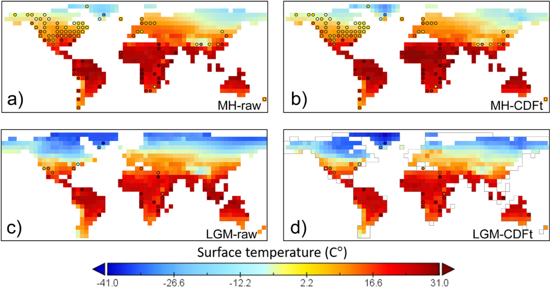
Figure 5. MH (a), (b) and LGM (c), (d) modelled temperature values (gridded map) and proxy-derived temperature values resampled to T21 grid using the aggregated average resampling method (data points in circles, Kaufman et al 2020) before correction (raw) and after correction (CDF-t) on T21 grid. Grey line in the (d) sub-figure represents the LGM land/sea mask (supplementary figure 1). The figure with reference data before resampling can be found in supplementary materials (supplementary figure 9).
