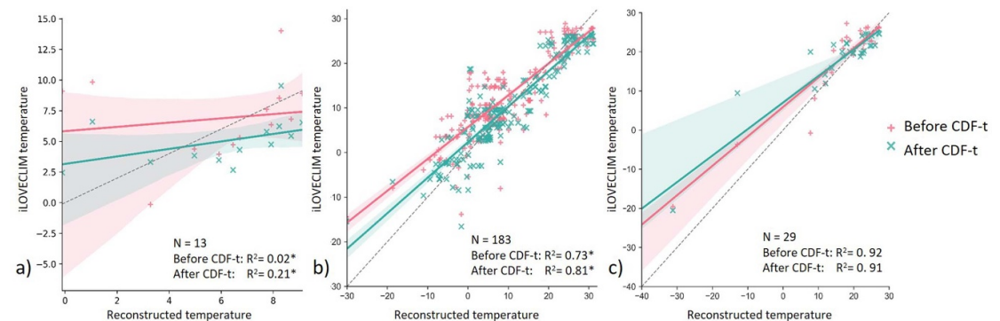
Figure 2. Simulated and reconstructed (Kaufman et al 2020) temperatures with fitted regression line and 95% confidence interval for (a) MH on the hi-res grid over Europe, (b) MH on a T21 grid globally, and (c) LGM on a T21 grid globally. Dashed grey line is the 1:1 line. A “*” marks when differences between the data before and after the CDF-t bias correction is significant at the 0.05 level (paired student's t -tests).
