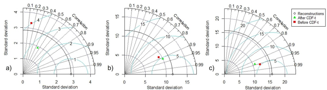
Figure 3. Taylor diagram representing (a) MH temperature on the hi-res grid over Europe, (b) MH on a T21 grid globally, and (c) LGM on a T21 grid globally before and after the CDF-t application. The simulated values are plotted against the reconstructed (Kaufman et al 2020) temperatures. Blue contours represent RMSE values.
