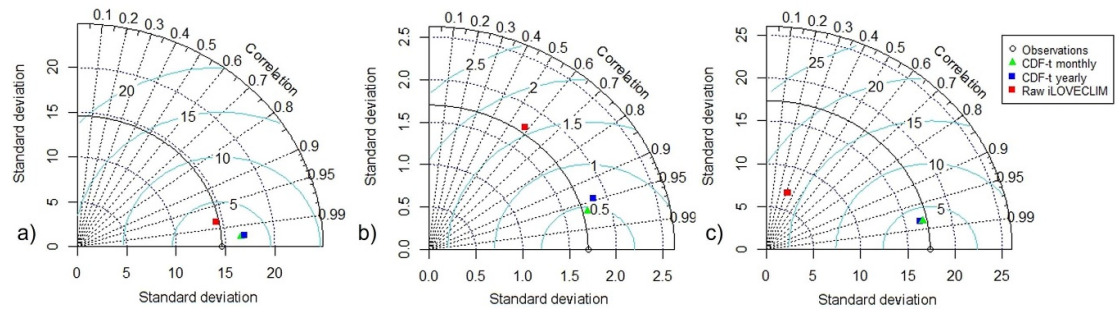
Figure 1. Taylor diagram representing (a) temperatures, (b) precipitations, and (c) relative humidity values of the pre-industrial time period before (Raw iLOVECLIM) and after the CDF-t application using yearly-based (CDF-t yearly) and monthly-based (CDF-t monthly) approach. The simulated values are plotted against the observations: Earth2Observe, WATCH Forcing Data (WFDEI), and ERA-Interim reanalysis data Merged and Bias-corrected for the InterSectoral Impact Model Intercomparison Project (Lange 2018). Blue contours represent RMSE values.
