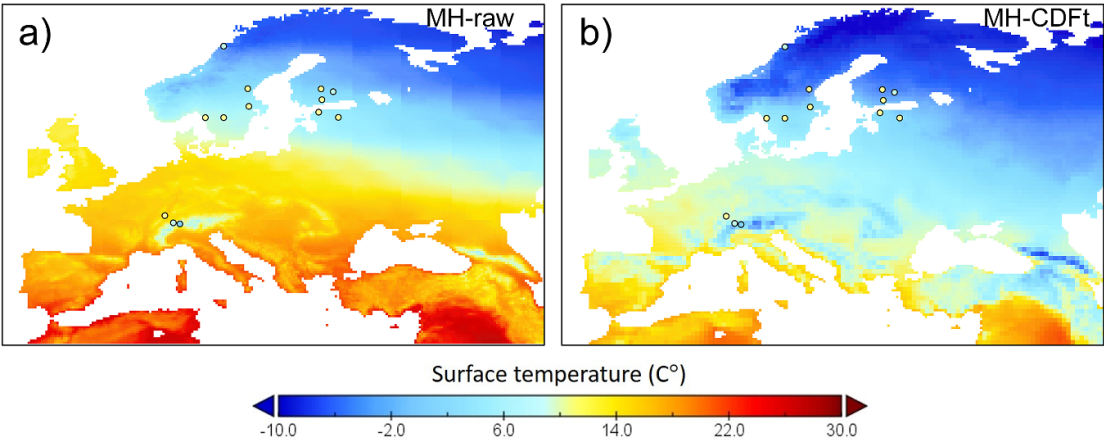
Figure 4. MH modelled temperature values (gridded map) and proxy-derived temperature values resampled to hi-res grid, using the aggregated average resampling method (data points in circles, Kaufman et al 2020) (a) before correction (MH-raw) and (b) after correction (MH-CDF-t) on hi-res grid.
