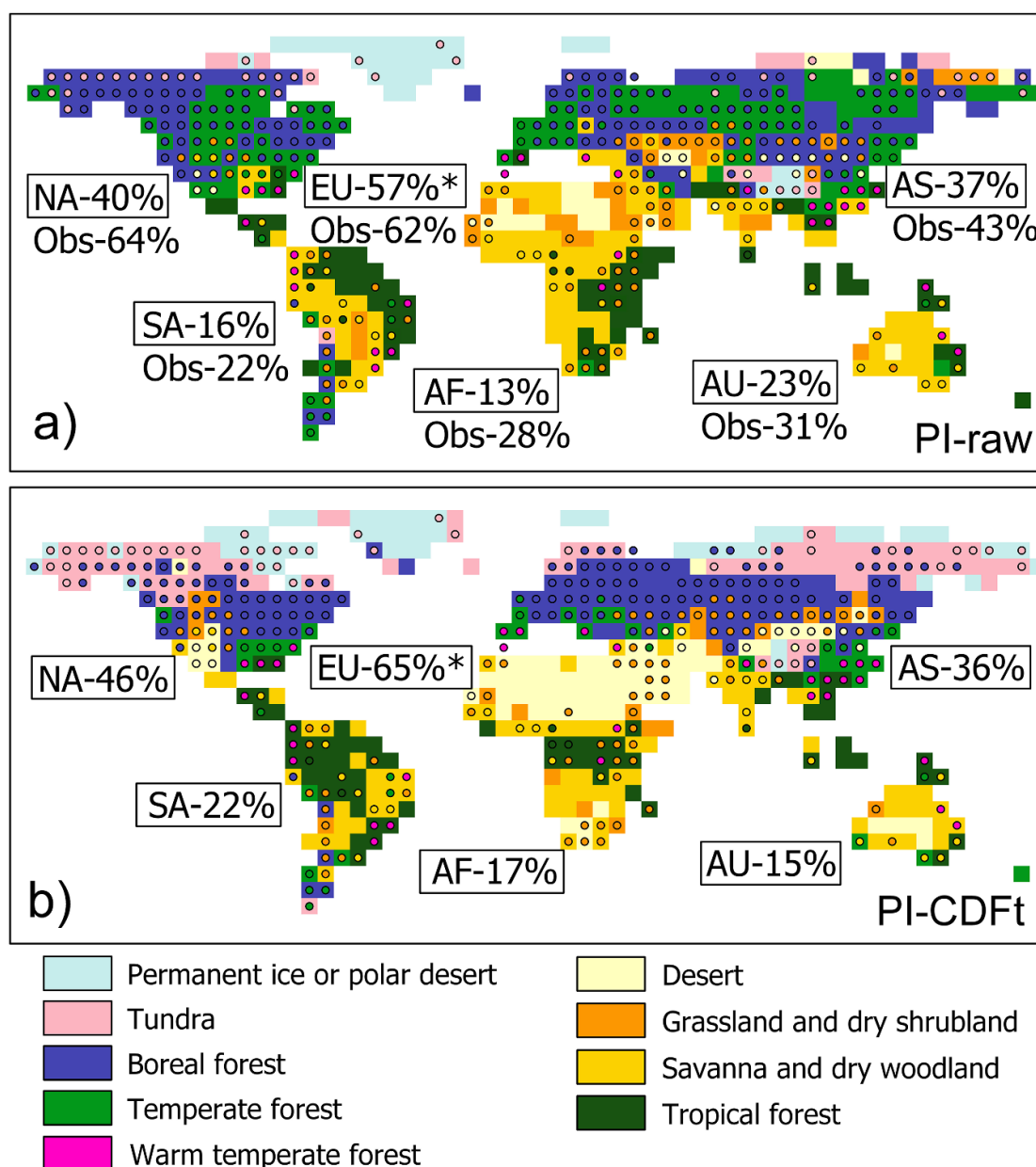
Figure 6. Model-data comparison of the biome distribution simulated from offline CARAIB run forced with iLOVECLIM climatic results for (a) pre-industrial on T21 grid before and (b) after the CDF-t correction. The superimposed circles are the data from the BIOME6000 Version 4.2 reconstruction resampled to the T21 grid using the majority resampling method. The biome classification of CARAIB has been adapted to match the megabiomes of BIOME6000. Matching ratios are presented in % per continent between megabiomes in pollen reconstructions (BIOME6000) and biomes predicted by the CARAIB model. NA—North America; SA—South America; EU—Europe; AF—Africa; AU—Australia; AS—Asia; Obs—CARAIB results with the use of the EWEMBI climatic variables (observations) as an input (control). A ‘*’ marks when differences between the data before and after the CDF-t bias correction is statistically significant at the 0.05 level with a chi-squared test. The figure with reference data before resampling can be found in supplementary materials (supplementary figure 10).
