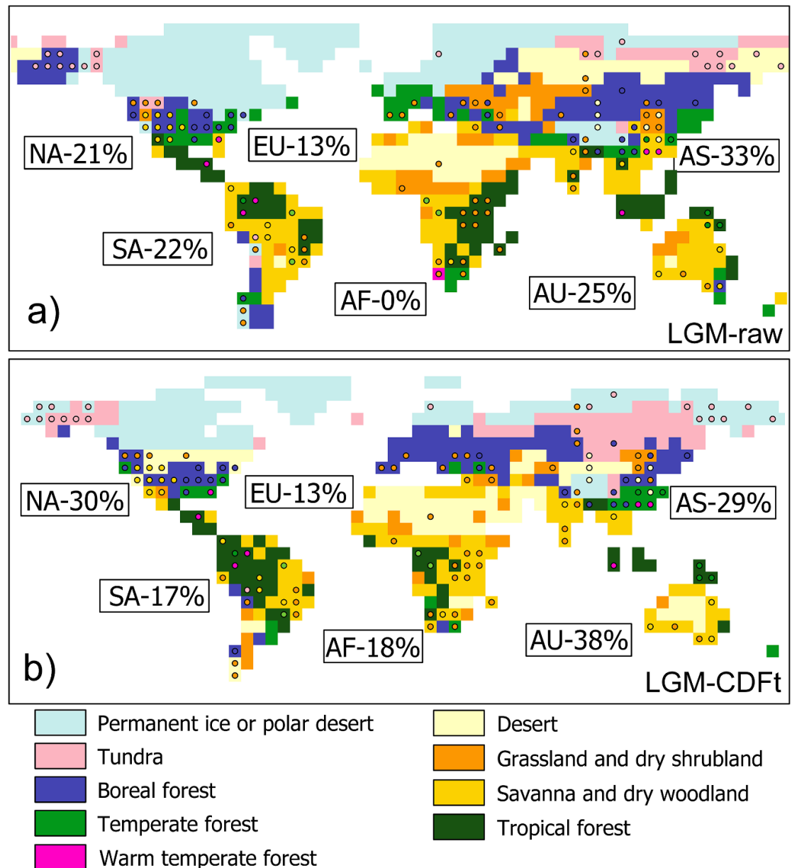
Figure 8. Model-data comparison of the biome distribution simulated from offline CARAIB run forced with iLOVECLIM climatic results for (a) LGM on T21 grid before and (b) after the CDF-t correction. The superimposed circles are the data from the BIOME6000 Version 4.2 reconstruction resampled to the T21 grid using the majority resampling method. The biome classification of CARAIB has been adapted to match the megabiomes of BIOME6000. Matching ratios are presented in % per continent between megabiomes in pollen reconstructions (BIOME6000) and biomes predicted by the CARAIB model. NA—North America; SA—South America; EU—Europe; AF—Africa; AU—Australia; AS—Asia; Obs—CARAIB results with the use of the EWEMBI climatic variables (observations) as an input (control). A ‘*’ marks when differences between the data before and after the CDF-t bias correction is statistically significant at the 0.05 level with a chi-squared test. The figure with reference data before resampling can be found in supplementary materials (supplementary figure 12).
