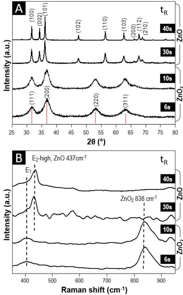
Figure 1. Evolution of (A) X-Ray diffraction patterns and (B) Raman spectra of Zn-based materials as a function of residence time ( t_R ).
