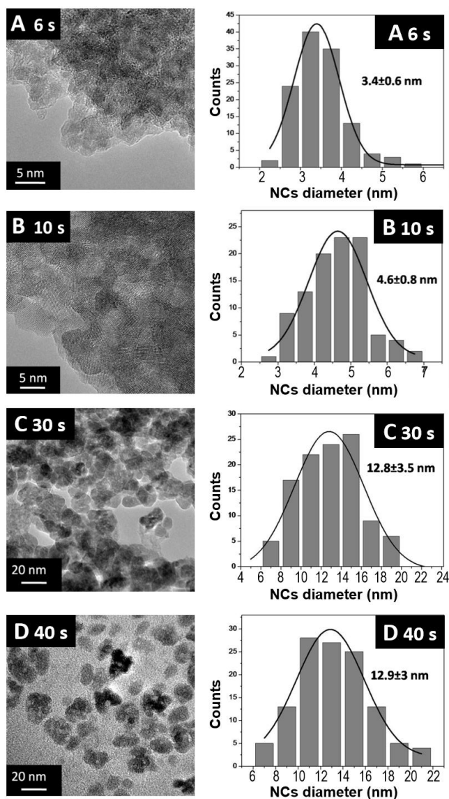
Figure 5 HRTEM micrographs of ZnO 2 nanoparticles and corresponding histograms for the samples obtained with a residence time of (A) 6 s, (B) 10 s, (C) 30 s and (D) 40 s.
