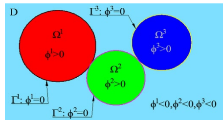
Fig. 23 A schematic diagram of the design domain which includes three level set functions. Permission to reprint from Elsevier copyright 2016 [143].
