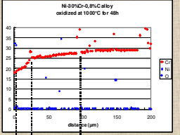
Cr content profiles obtained by microprobe analysis through the zone affected by oxidation
