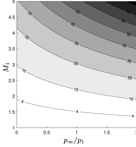
Fig. 2 Critical angle \alpha_c as function of the upstream shock Mach number M_1 and the parameter bp_1
