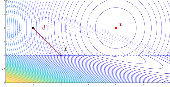
Figure 2.1: The level curves of \theta in counter-example 2.4 with \mu = 3 (and the dotted level curves of x \mapsto \frac{1}{2}\|Mx + q\|^2 ), the solution \bar{x} to the LCP, the current point x and the unfortunate NM direction d , which is an ascent direction of \theta .
