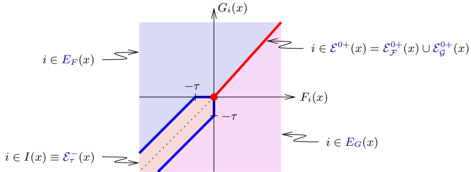
Figure 2.2: The pair (F_i(x), G_i(x)) determines which index sets E_F(x) , E_G(x) , or I(x) , i belongs to; see (2.14) for the definition of these index sets. The nondifferentiability of H_i can only occur on the main diagonal, at points x for which F_i(x) = G_i(x) . Nevertheless the secure PNM direction (2.13) carefully deals with points that are near an x such that F_i(x) = G_i(x) < 0 , those with a pair (F_i(x), G_i(x)) inside the fork in the left-bottom part of the picture (it then replaces one equality defining the plain NM direction (2.1) by a pair of inequalities). The width of this fork is controlled by the kink tolerance \tau > 0 , which can be taken very small in practice, in order to avoid having too many inequalities in (2.13).
