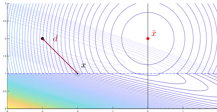
Figure 2.1: The level curves of \theta in counter-example 2.3 with \mu = 3 (and the dotted level curves of x \mapsto \frac{1}{2}\|Mx + q\|^2 ), the solution \bar{x} to the LCP, the current point x and the unfortunate NM direction d , which is an ascent direction of \theta .
