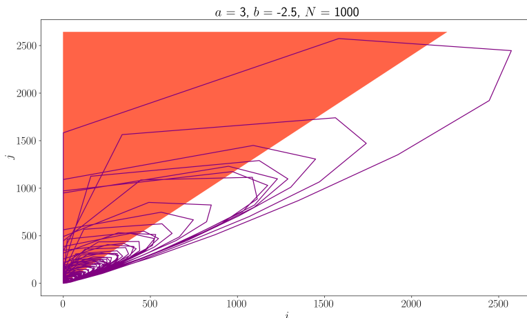
FIGURE 3. An illustration of Case \mathcal{R}_2 . Here, the parameters are a = 3, b = -2.5 and N = 1000 . In red, the set A of couples (i, j) such that s_{ij} = s_{0i} = 0 .
