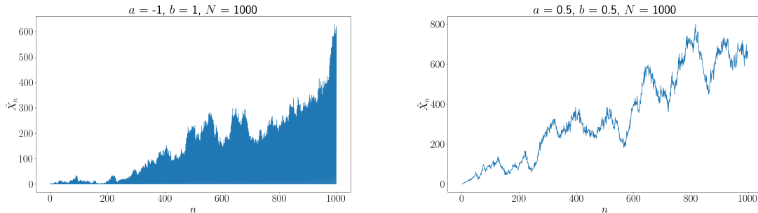
FIGURE 7. Trajectories of (\tilde{X}_n)_{0 \leq n \leq 1000} for critical parameters (a, b) = (-1, 1) on the left and (a, b) = (0.5, 0.5) on the right. We observe a linear growth of the process as it could be expected in critical cases.
