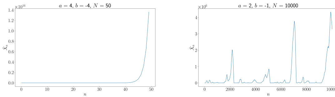
FIGURE 8. Trajectories of (\tilde{X}_n)_{0 \leq n \leq 10000} for critical parameters (a, b) = (4, -4) on the left and (a, b) = (2, -1) on the right.
