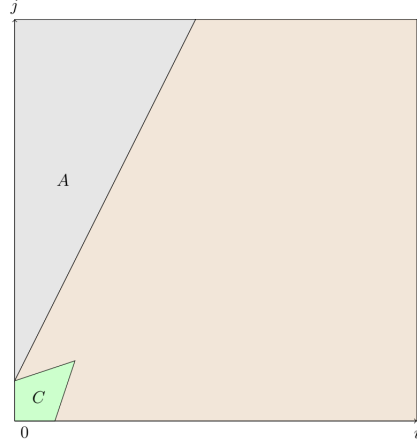
FIGURE 4. Graphical representation of the sets A, C described above.
