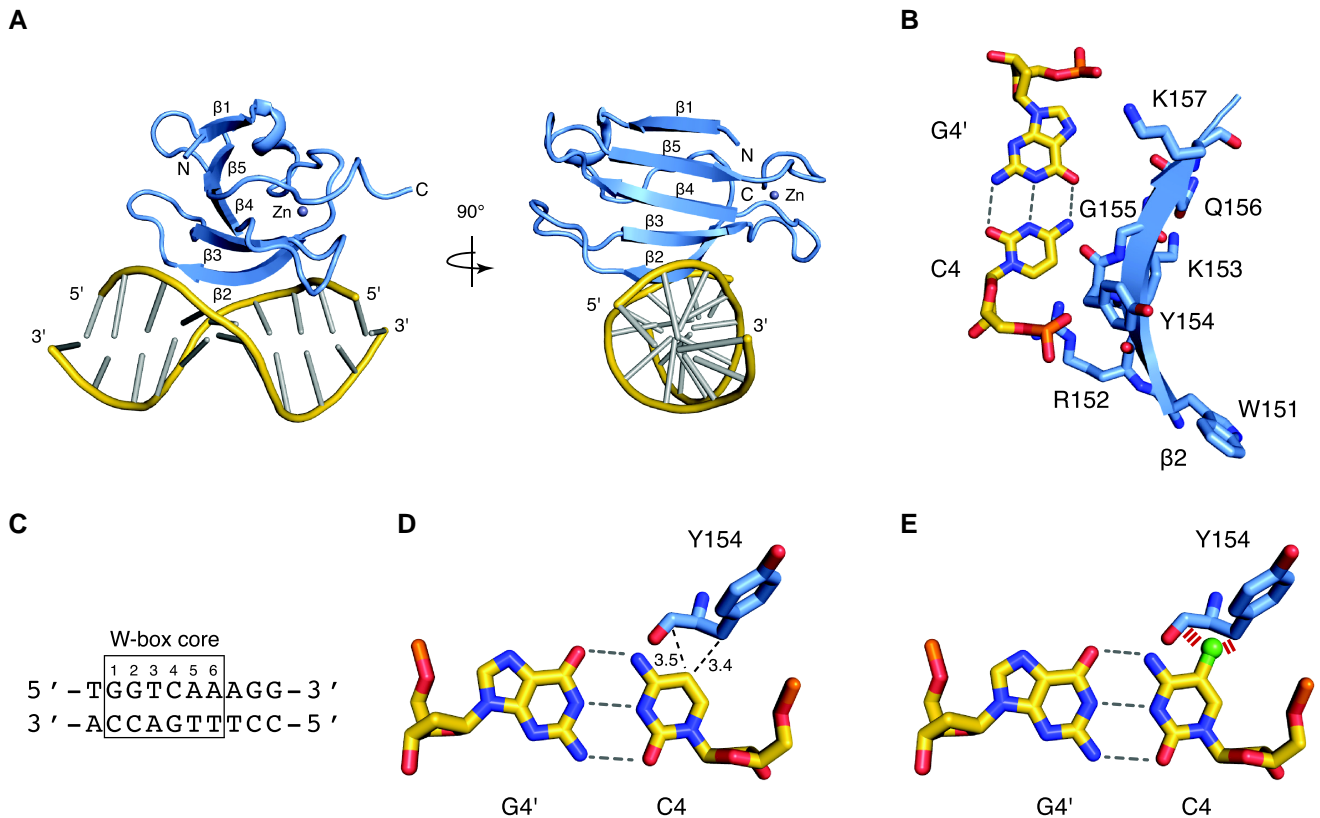
Figure 3. Structural model of the AtWRKY40 DBD in complex with a W-box DNA duplex. A) Lowest energy structure from the ensemble of models of the complex between AtWRKY40 and the W-box element of panel C. The protein is shown as a cartoon in light blue, the five \beta -strands are labelled, and the zinc ion is shown as a grey dot. The DNA backbone is shown as a cartoon in yellow and the base-pairs are shown with the ladder representation in grey. B) Close-up view of the WRKY motif of \beta 2 (W151-K157). The protein is shown in light blue with the side chains represented as sticks. The C4-G4' DNA base-pair is shown as sticks in yellow. The \beta 2 strand enters deeply into the DNA major groove at the level of the C4-G4' base-pair. In particular, the aromatic ring of C4 makes van der Waals contacts with the side-chain of Y154. C) Sequence of the DNA W-box element used for modelling the interaction of AtWRKY40 with DNA. D) The position 5 of C4 makes van der Waals contacts with Y154. E) Modelling a methyl group (in green) onto unmodified C4 from the W-box core reveals steric hindrance (indicated with red strips) with Y154.
