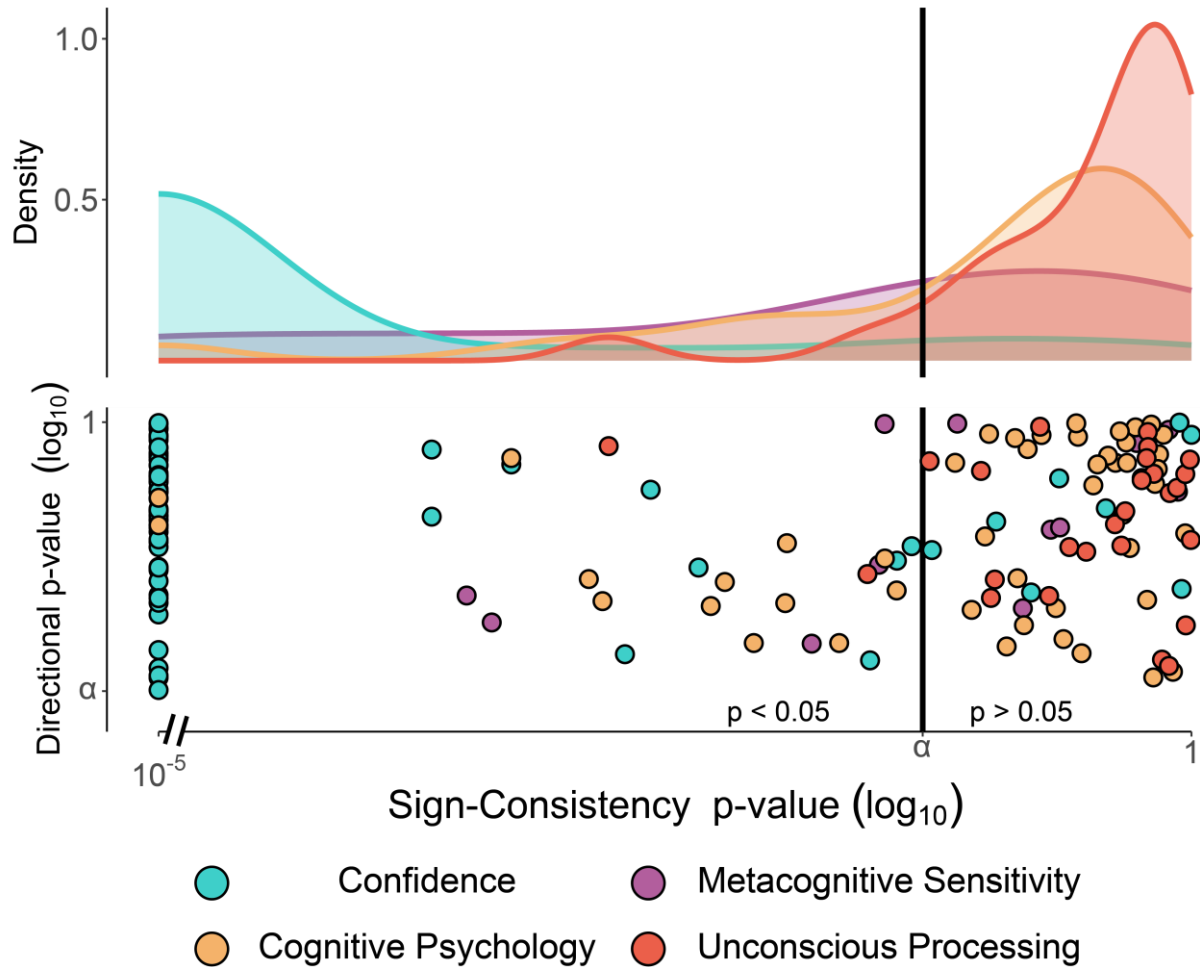
Figure 4. Sign consistency test results for null directional effects from different cognitive psychology fields. Turquoise and purple markers indicate the outcomes for datasets from the Confidence Database (Rahnev et al., 2020) that were analysed to reveal differences in confidence and metacognitive sensitivity between responses, respectively. Orange markers indicate the outcomes for effects from various cognitive psychology studies. Finally, for comparison purposes, we also plot here in red the results of the studies on unconscious processing (N=26), reported in the previous section. Lower panel: each point depicts the \log_{10} transformed p-values obtained by the sign consistency test (x-axis) and a directional sign-flipping test (y-axis; datasets were filtered to exclude significant directional effects, hence the minimal directional p-value for all datasets is \alpha = .05 ). Upper panel: The p-values density distributions that summarize the results in the lower panel for datasets in each field.
