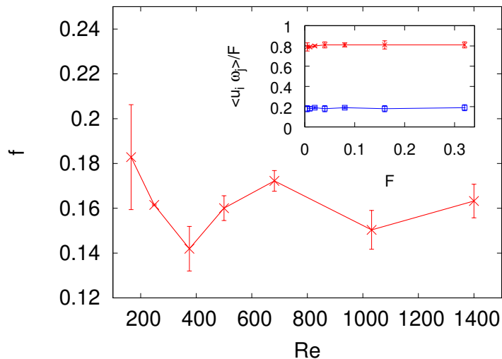
FIG. 7. Friction factor f = F/(KU^2) as a function of the Reynolds number Re = U/(\nu K) . Errors are estimated from the fluctuations of the amplitude of the average velocity profile. Inset: relative contribution of the quadratic terms to the momentum budget of Eq. (2), normalized by the forcing amplitude. The red upper line corresponds to the contribution from the advection terms \overline{u_i \omega_i} , the blue lower one to that from the vortex stretching terms \overline{\omega_i u_z} .
