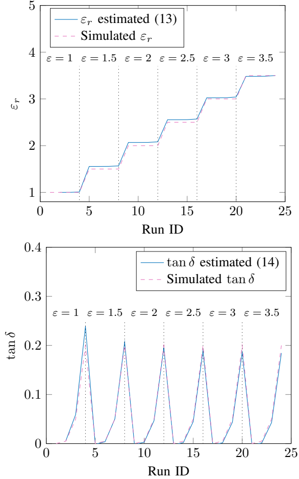
Fig. 5. \epsilon_r and \tan \delta estimated with (13) and (14) respectively. The different values used for the study and corresponding to a ID number are shown in Table I.
