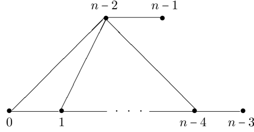
Figure 6.2: The graph Q_n
