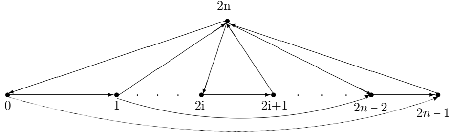
Figure 1.2: The tournament T_{2n+1}
