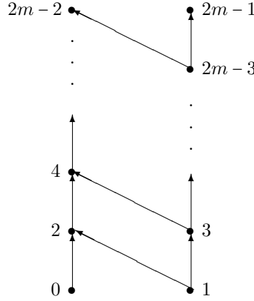
Figure 4.3: The partial order R_{2m}
