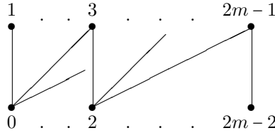
Figure 4.1: The half-graph H_{2m}
