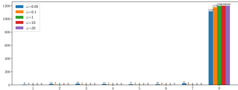
Figure 11: Distribution of \hat{\eta}^N(T, x) . The domain x \in [-3, 4] is computed for 1200 samples over a discrete grid of 100 points, i.e. mesh 8 \cdot 10^{-2} , N = 2^5, 2^6, \dots, 2^{16} for \ell = 7 . The method tends to pick the largest bandwidth.
