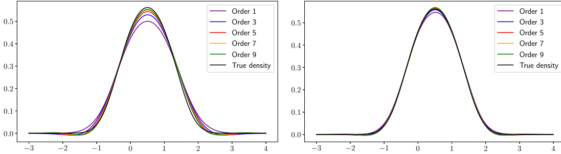
Figure 10: Reconstruction of \mu_T by \hat{\mu}_T^{N,h,\hat{\eta}^N(T,\cdot)} with \varpi = 23 , for different kernel orders for N = 2^{10} (Left) and N = 2^{15} (Right). Higher order kernels outperform the reconstruction provided with standard Gaussian kernels ( \ell = 1 ) for N = 2^{10} .
