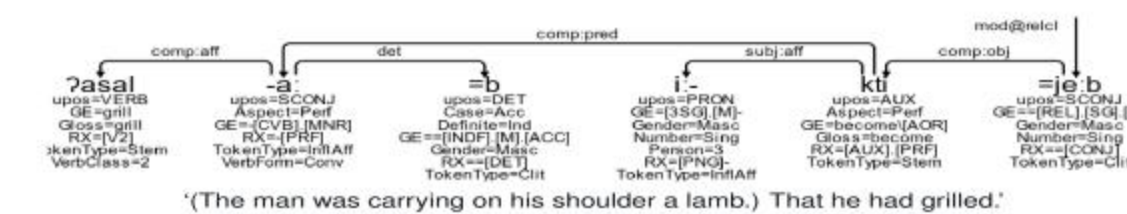
Fig. 8: SUD style relative clause construction
