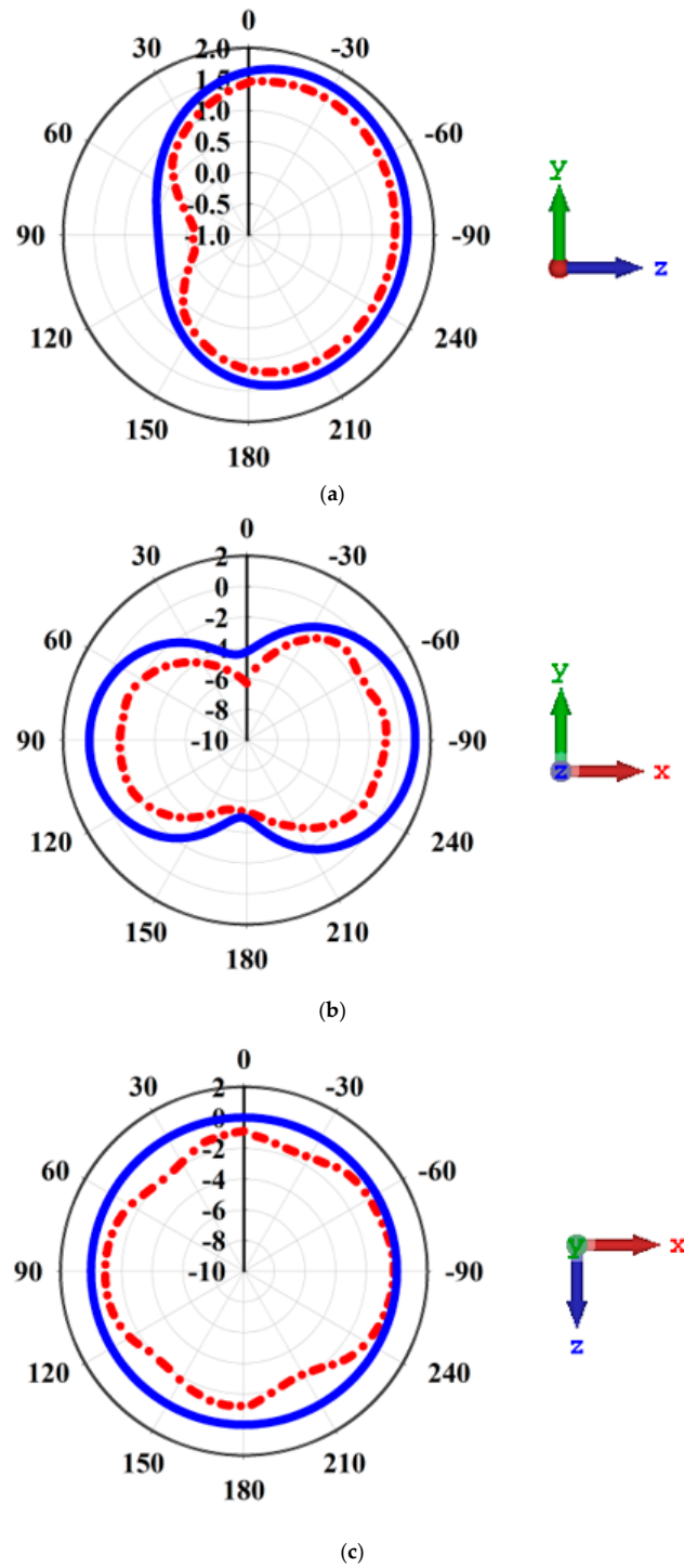
Figure 10. Two-dimensional simulated and measured radiation patterns at 2.4 GHz for planes: (a) YZ ( \varnothing = 90^\circ ), (b) XY ( \theta = 90^\circ ), (c) XZ ( \varnothing = 0^\circ ).
