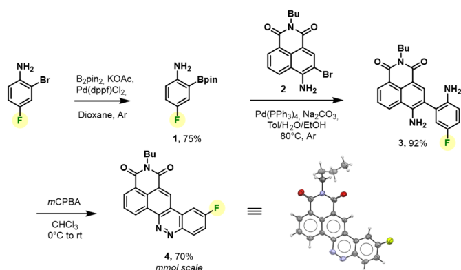
Figure 2. mmol scalable synthesis and X-ray diffraction structure of bench stable CinNaphth-F 4 .
