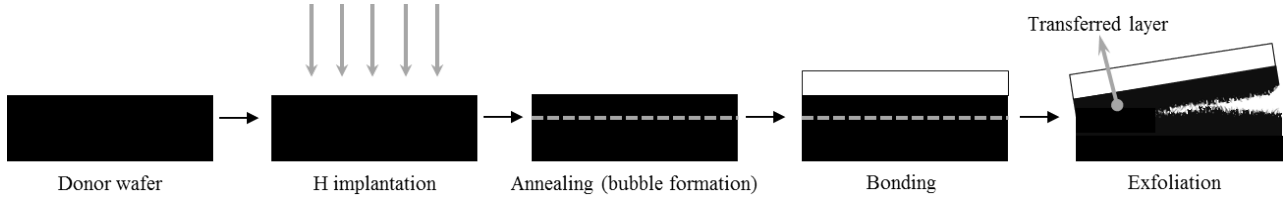
Fig. 1: Technological steps conventionally used in a Smart-Cut process. The main steps consist of hydrogen implantation inside a donor wafer, an annealing to induce bubble formation, a bonding to a receiving wafer and a fracture treatment that enables the material splitting parallel to the donor surface.
