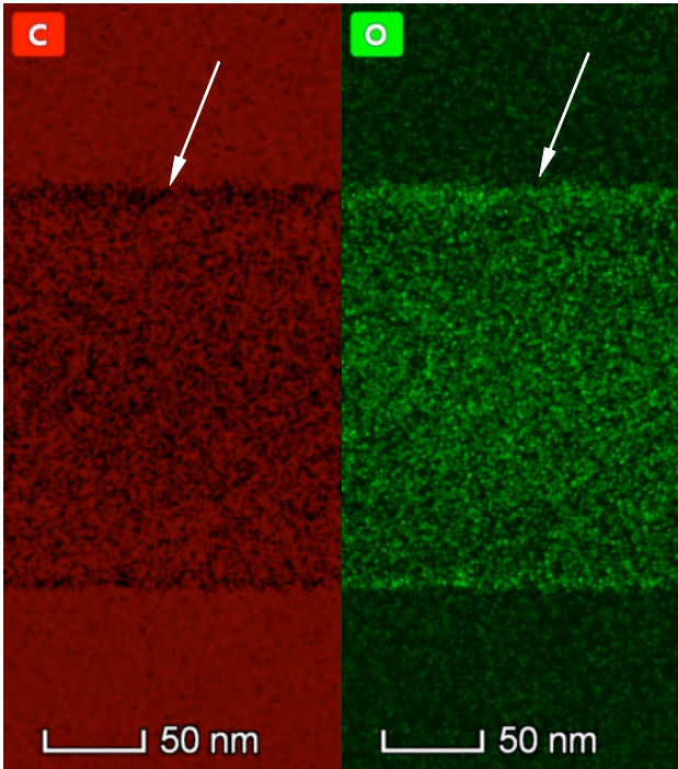
Fig.6: Carbon and oxygen EDS maps obtained in the FIB lamella prepared in the HD region. Layers a-b-c, presented in Fig.4, are revealed. A decrease of the C content is evidenced in layer (b). White arrows indicates the interface of the (a) and (b) layers, highlighting a strong decrease of the C content (while an increase of the O content is revealed).
