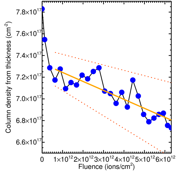
Fig. C.2. \text{CH}_3\text{CN} column-density evolution as estimated from equation B.2 as a function of 39.25 MeV ^{56}\text{Fe}^{10+} ion fluence, with the thickness retrieved from the models presented in Fig. B.1.
