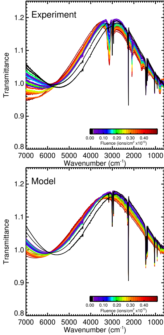
Fig. C.1. Acetonitrile infrared spectra and modelling. Upper panel: Infrared transmittance spectra of a \text{CH}_3\text{CN} ice-film evolution as a function of 39.25 MeV ^{56}\text{Fe}^{10+} ion fluence. Lower Panel: Model spectra fitted to the data as a function of fluence. See text for model details.
