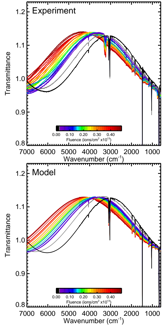
Fig. B.1. Benzene infrared spectra and modelling. Upper panel: Infrared transmittance spectra of a \text{C}_6\text{H}_6 ice film evolution as a function of 39.25 \text{ MeV } ^{56}\text{Fe}^{10+} ion fluence. Lower Panel: Model spectra fitted to the data as a function of fluence. See text for model details.
