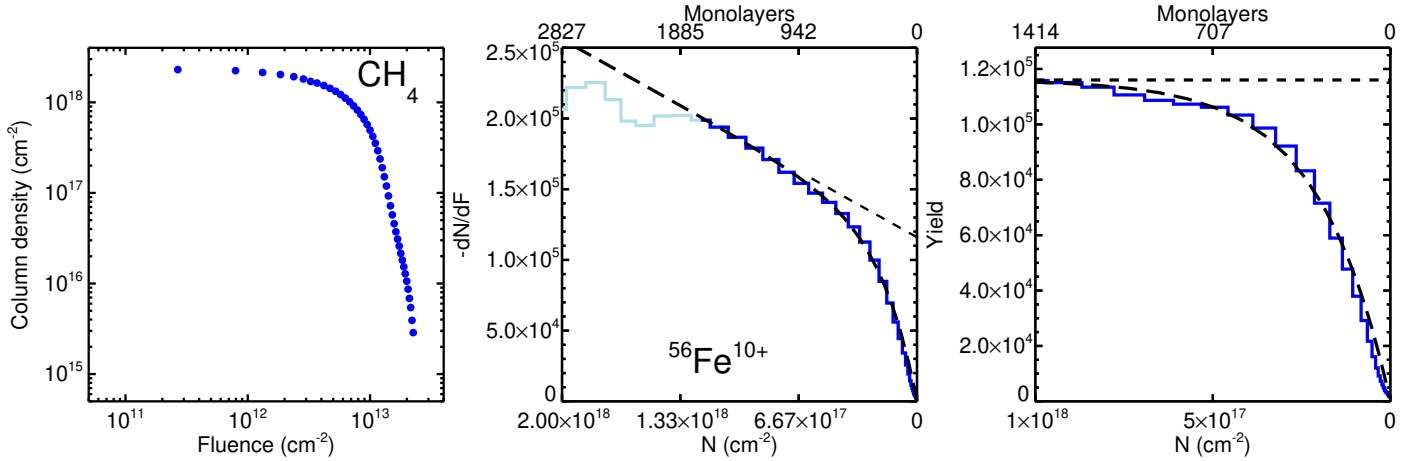
Fig. A.2. \text{CH}_4 sputtering yield determination. Left panel: \text{CH}_4 column-density evolution measured with the \nu_4 mode spectra as a function of ^{56}\text{Fe}^{10+} ion fluence for a \text{CH}_4 ice film deposited and measured at 10 K. Middle panel: Experimentally measured differential evolution of -\text{dN}/\text{dF} as a function of column density, to be compared to equation A.1. A fit of the equation to the data is shown as a black long-dashed line, and a fit not taking into account the finite depth of sputtering is shown with a short-dashed line. Right panel: Sputtering yield evolution as a function of column density; over-plotted are the infinite thickness yield (dashed lines) and adjusted exponential decay (long-dashed lines). See text for details.
