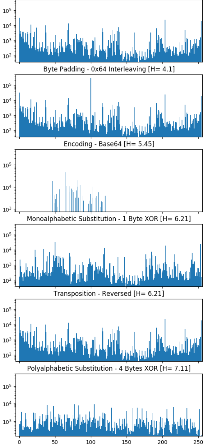
Fig. 4. Byte Frequency Distribution w.r.t. Schemes Original [H= 6.21]
