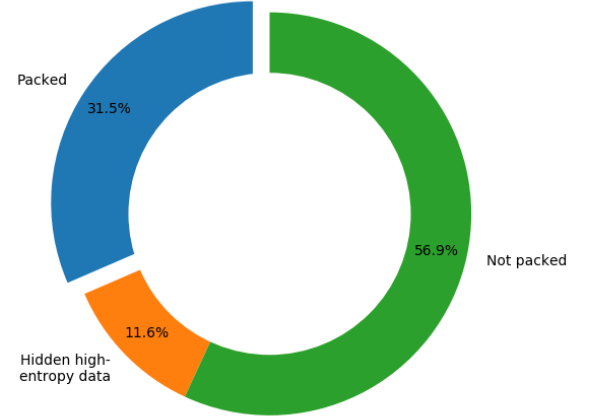
Fig. 3. Dataset composition (cardinality = 46,295)
