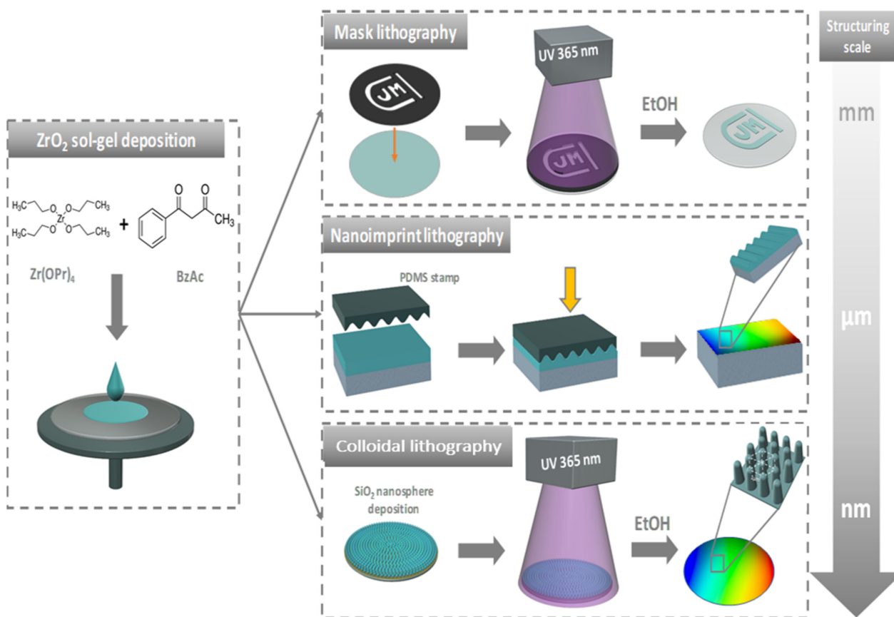
Figure 7. Illustration of the different methods of ZrO 2 sol-gel micro-nanostructuring.
