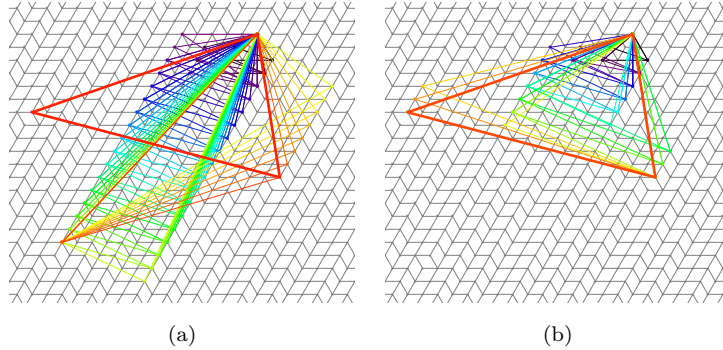
Figure 2: The evolution for normal (1, 73, 100) with H-algorithm (a) and R-algorithm (b). Here, L-algorithm has the same output as the R-algorithm. Every triangle of the evolution is superimposed. The initial triangle is blue. The last one is red.
