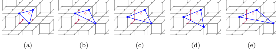
Figure 1: The evolution (from left to right) of a tetrahedra-based plane-probing algorithm on a digital plane of normal (1, 2, 5) .
