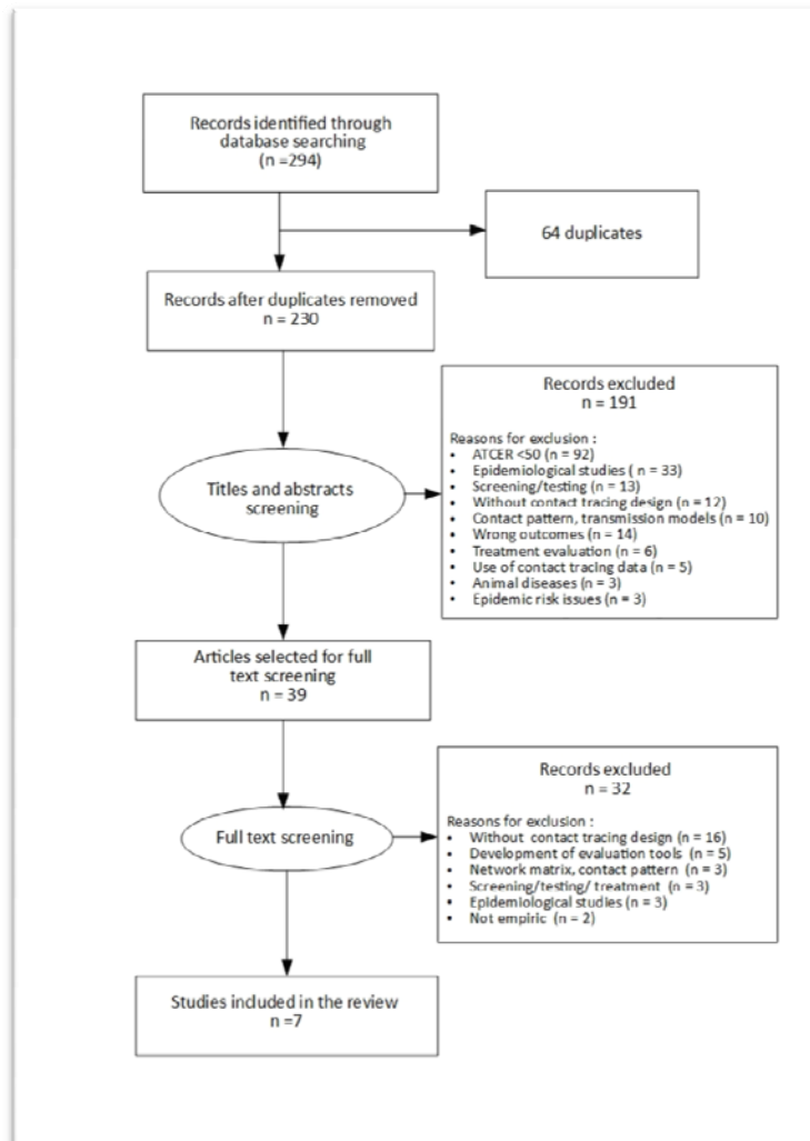
Figure 1: PRISMA diagram
