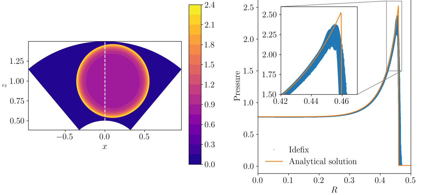
Fig. 5. Sedov–Taylor blast wave in spherical geometry at t = 0.1 . The blast is initialized slightly off the polar axis (at x = 0.1, z = 1 ). Left panel: slice of the pressure field through y = 0 . The dashed white line represents the polar axis of the domain, which is regularized automatically by IDEFIX. Right panel: pressure distribution as a function of the distance from the blast center. The inset shows a zoom around the blast shock region.
