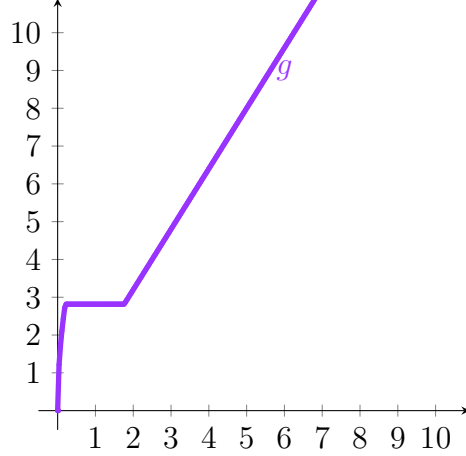
FIGURE 2.1. graph of g for (K, h, \varepsilon) = (-1, 1.6, 0.2)
