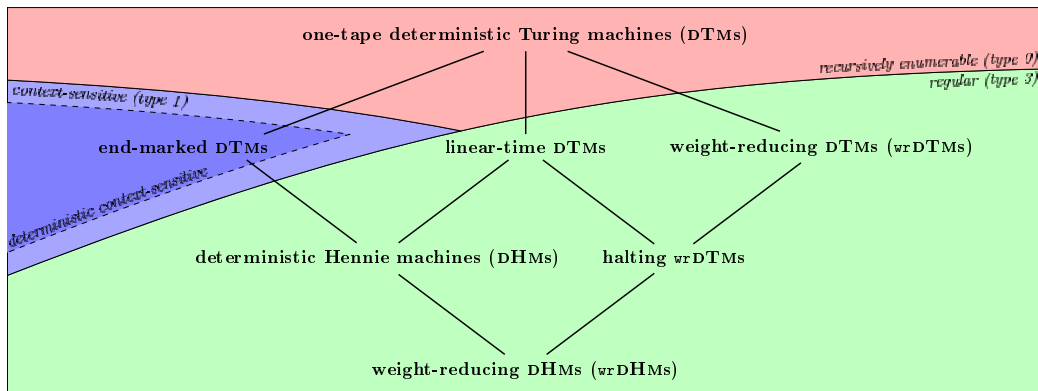
Figure 1: Variants of one-tape deterministic Turing machines and their expressive power confronted with the Chomsky hierarchy. In particular, end-marked DTMs are known as deterministic linear bounded automata in the literature, and recognize the so-called deterministic context-sensitive languages , a subclass of context-sensitive languages, see [29]. It is still unknown if such inclusion is strict.
