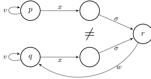
Fig. 4. The strong forbidden pattern: v \in \Sigma^+ , x \in \Sigma^* , \sigma \in \Sigma , w \in \Sigma^* .
