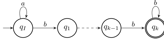
Fig. 1. The minimum automaton accepting the language a^*b^k b^* .
