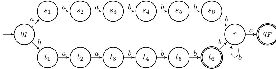
Fig. 6. The minimum automaton A_{4,6} accepting the language L_{4,6} .
