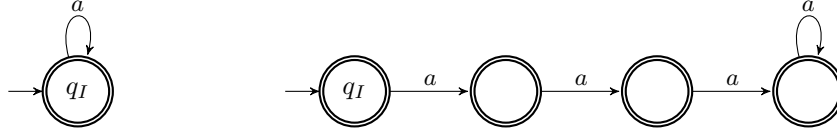
Fig. 3. The minimum DFA accepting the reversible language a^* , and an equivalent DFA containing the 3-forbidden pattern
