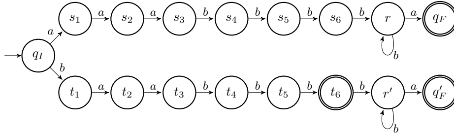
Fig. 7. A REV 5 DFA accepting the language L_{4,6} .
