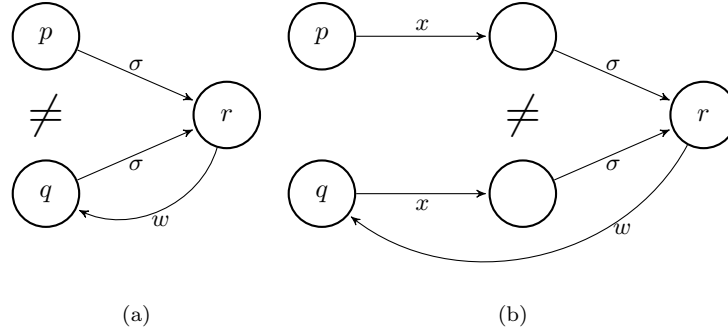
Fig. 2. The forbidden pattern (a) and the k -forbidden pattern (b), in which \sigma \in \Sigma , w \in \Sigma^* , and x \in \Sigma^{k-1} .
