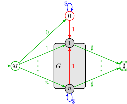
Fig. 9. The automaton A obtain from a graph G . Only transitions that have been added to G (i.e., transitions (ii) to (v)) are depicted.
