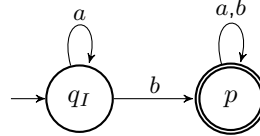
Fig. 5. The minimum automaton accepting the language L = a^*b(a+b)^*
