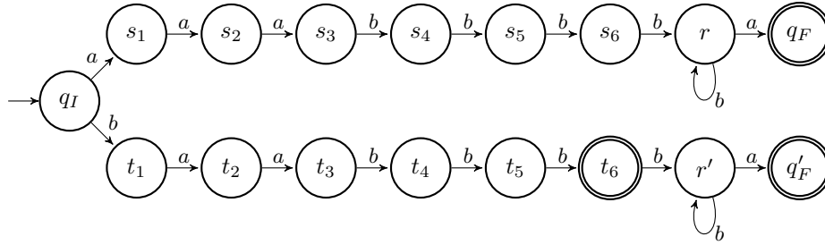
Fig. 7. A REV 5 DFA accepting the language L_{4,6} .
