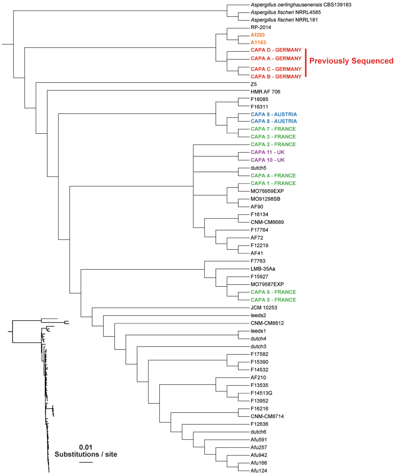
FIG 1 Phylogeny of 55 A. fumigatus isolates and 3 outgroup taxa reveals that the 11 new CAPA isolates span the genomic diversity of the species. We used 4,515 single-copy orthologs from a total of 61 taxa (11 new CAPA isolates, three non- A. fumigatus outgroup strains, 43 A. fumigatus isolates that span the diversity of the species, and 4 previously analyzed CAPA isolates) as input to construct a maximum likelihood tree. A slight geographic clustering of CAPA isolates was observed, but isolates from different locales were more diverse than a previous set of four CAPA isolates (all of which were isolated from the same hospital in Germany).
