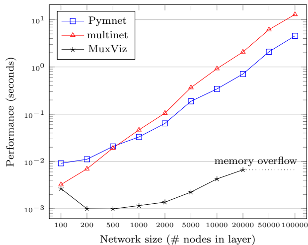
Fig. 1 Comparison of three multilayer network libraries for performance of two layer network aggregation over network size.
