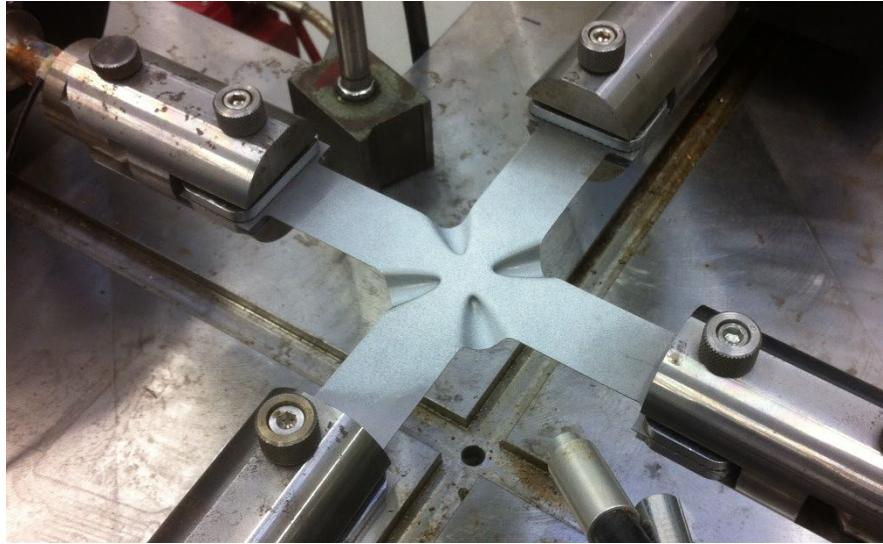
Fig. 4. Experimental setup with the pre-deformed cruciform sample.
