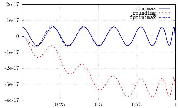
Fig. 1. Relative errors between \arctan(x) and approximations of the form r(x) = \sum_{i=0}^6 p_i x^{2i+1} / \sum_{i=0}^6 q_i x^{2i} on [0.00012207, 1] .
