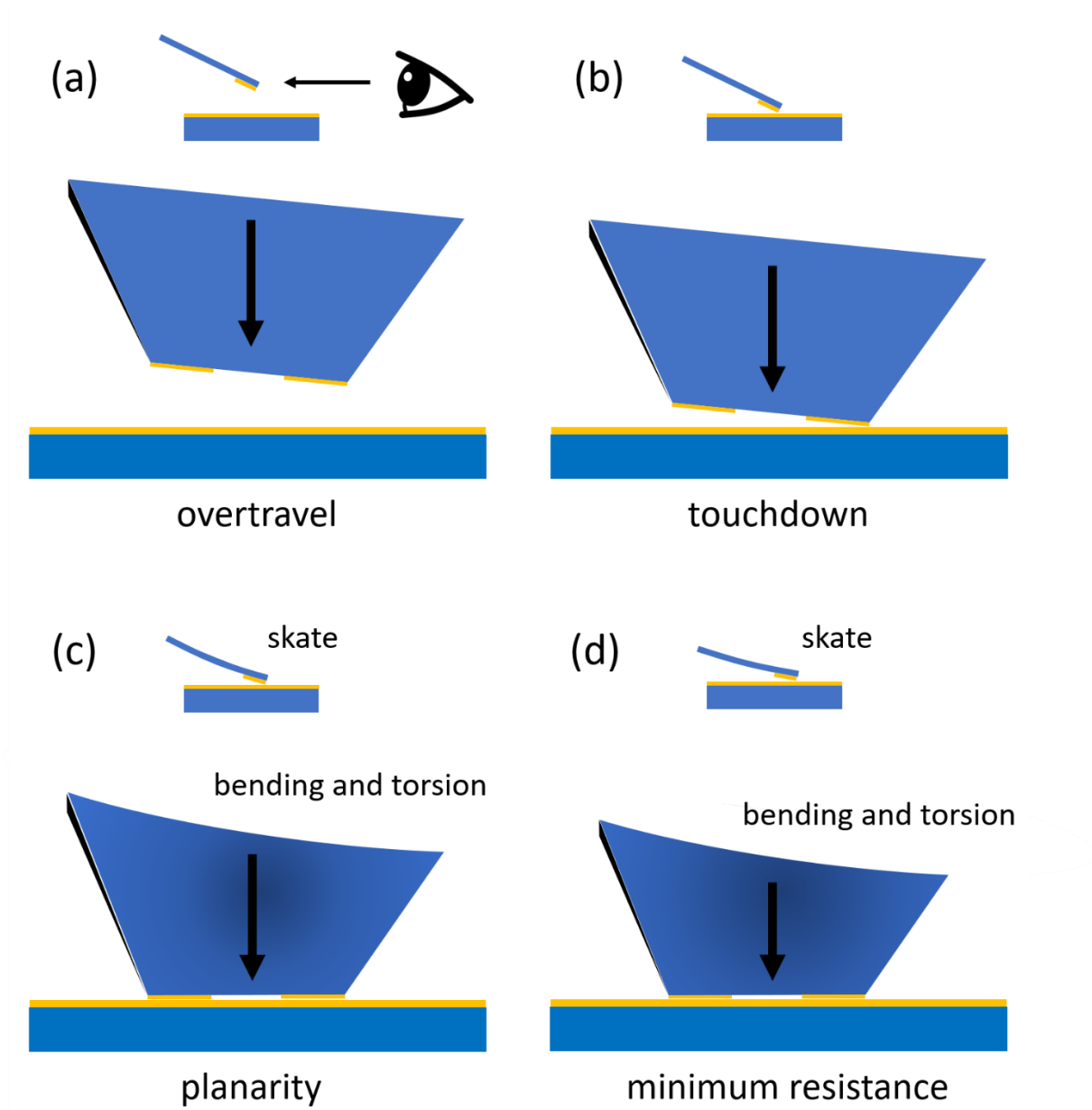
Figure 13. Schematic diagram showing torsional compensation of roll error angle in a flexible microcantilever-based probe. (a) Vertical downward overtravel. (b) Touchdown of right-hand contact pad with surface. (c) Further overtravel leads to bending and torsion of the cantilever to achieve apex planarity. (d) Further overtravel increases the contact force to achieve two low resistance contacts. The eye inset to (a) shows how one is looking at the apex of the cantilever in the figure.
