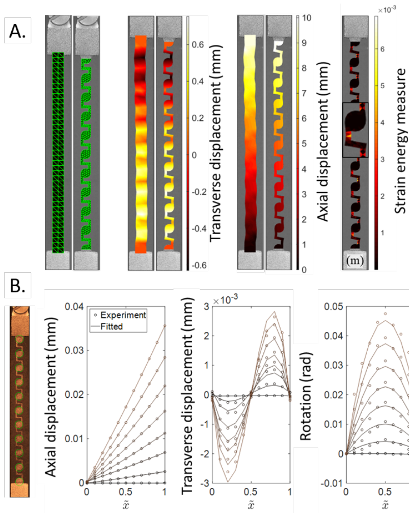
Figure 15. A. Macro-scale and micro-scale determination of beam deformation using DIC. B. Measured grain rigid body motions obtained from DIC and predicted kinematics of the chiral Cosserat beam model.
