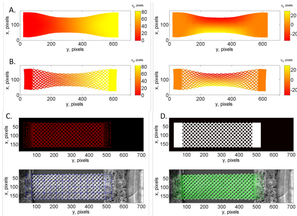
Figure 14. A. Macro-scale analyses using a second gradient theory. B. Micro-scale analyses using a first gradient theory. C. Results of the DIC backtracking for the macro-scale analyses. D. Results of the DIC backtracking for the micro-scale analyses.
