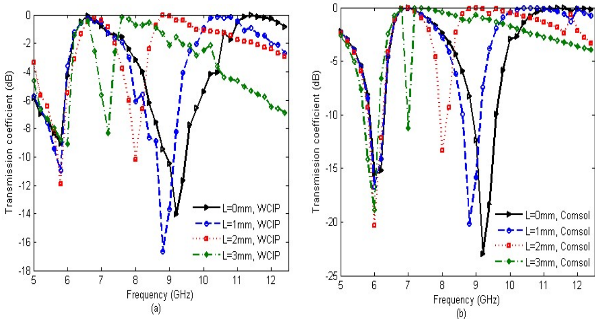
Fig. 9. Transmission coefficient S_{21} versus the operating frequency for different lengths L when the FSS is y -polarized. (a)WCIP results, (b) COMSOL results
