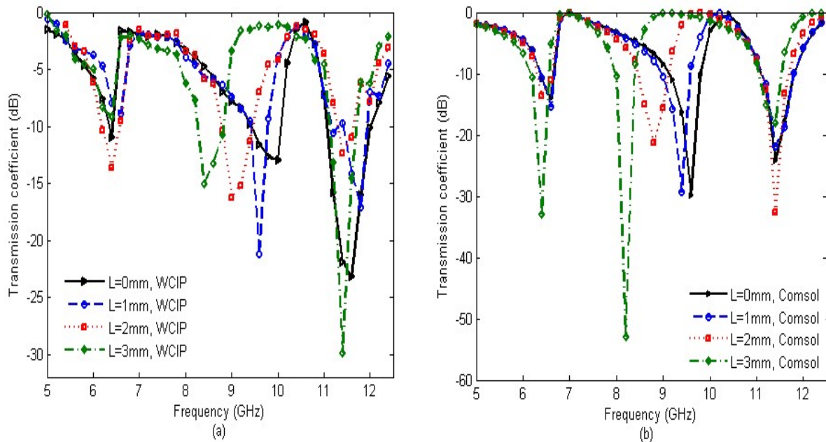
Fig. 8. Transmission coefficient S_{21} versus the operating frequency for different lengths L when the FSS is x -polarized. (a)WCIP results, (b) COMSOL results.
