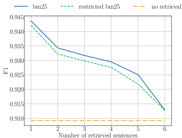
Figure 4: Mean F1 score versus number of retrieved sentences across 3 runs for the oracle version of the bm25 heuristic, and the same heuristic restricted to distant context.
