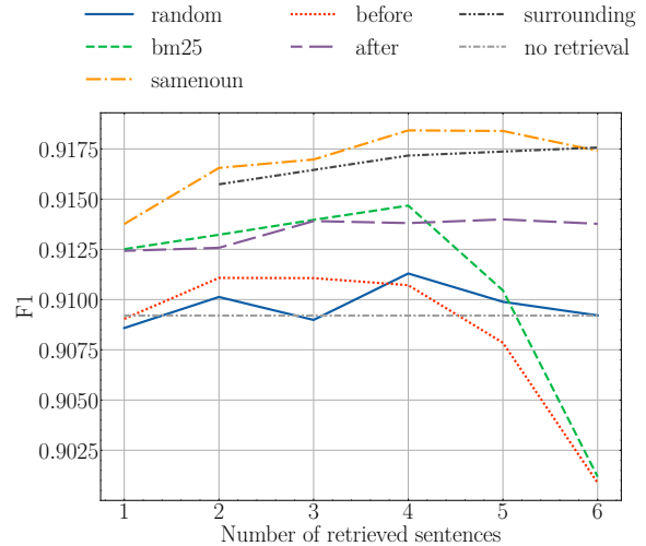
Figure 1: Mean F1 score versus number of retrieved sentences for all retrieval heuristics across 3 runs.
