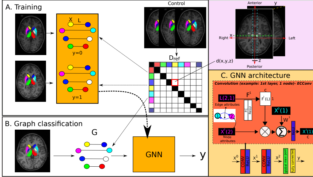
Fig. 1. Overview of the proposed GNN-based method for NAIS and PC detection
