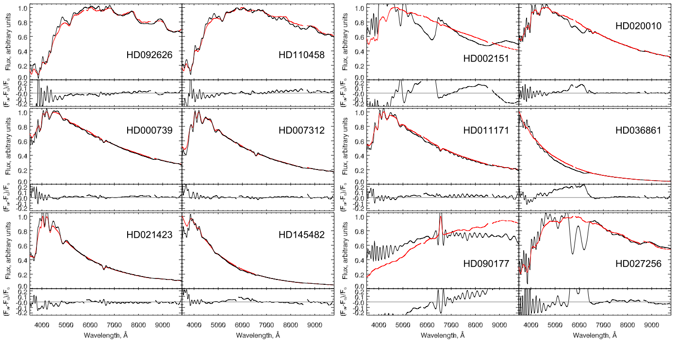
Figure 14. Examples of 12 resolution-degraded UVES-POP spectra (red) with Gaia BP/RP spectra (black) overlaid. All spectra are normalized to unity at the maximal flux of the convolved UVES-POP spectrum. Below each plot we show a panel with the fractional flux differences between the two spectra. The left six panels present the stars with a satisfactory agreement between UVES-POP and Gaia; the right six panels show stars with obvious calibration issues in the Gaia BP/RP spectra. None of the 12 stars have significant variability according to SIMBAD.
