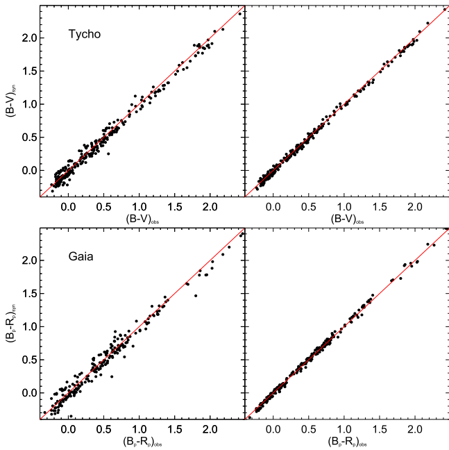
Figure 8. Top: comparison of the synthetic Tycho colors (B - V)_{\text{syn}} of the spectra corrected with observed colors (B - V)_{\text{obs}} before and after spectrophotometric correction (left and right panels, respectively). Bottom: same as the top panels, but for Gaia colors (B_p - R_p) .
