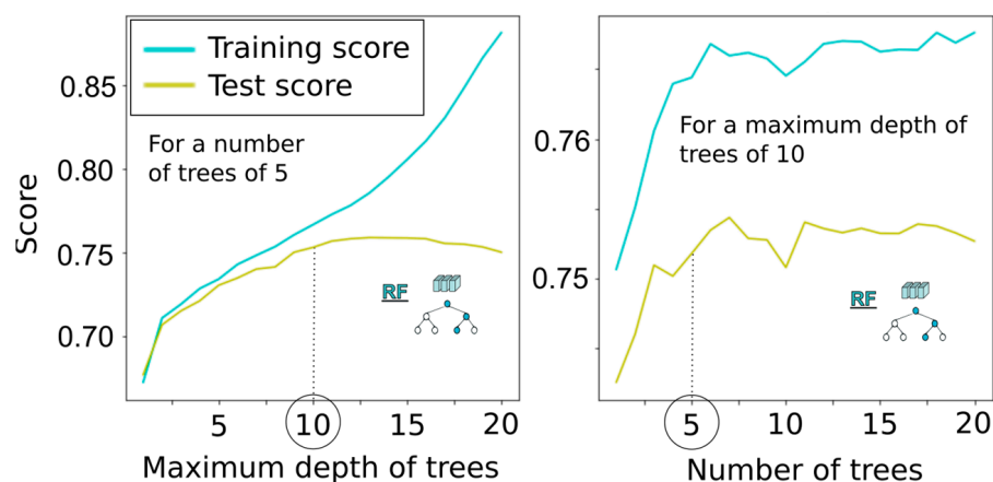
Figure 4. Training and test scores on Aude 1 sample for different maximum depths of trees ( left ) and numbers of trees ( right ) used in the RF algorithm. Setting a number of 5 trees along with a maximum depth of 10 provided a good compromise between performance and computational speed while avoiding overfitting (increasing training score but decreasing test score).
