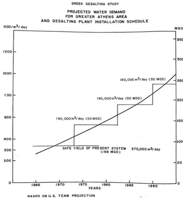
Figure 2: Water demand projections considering the installation of increasing desalting capacity for the OSW's 1966 Athens, Greece Water Study.
