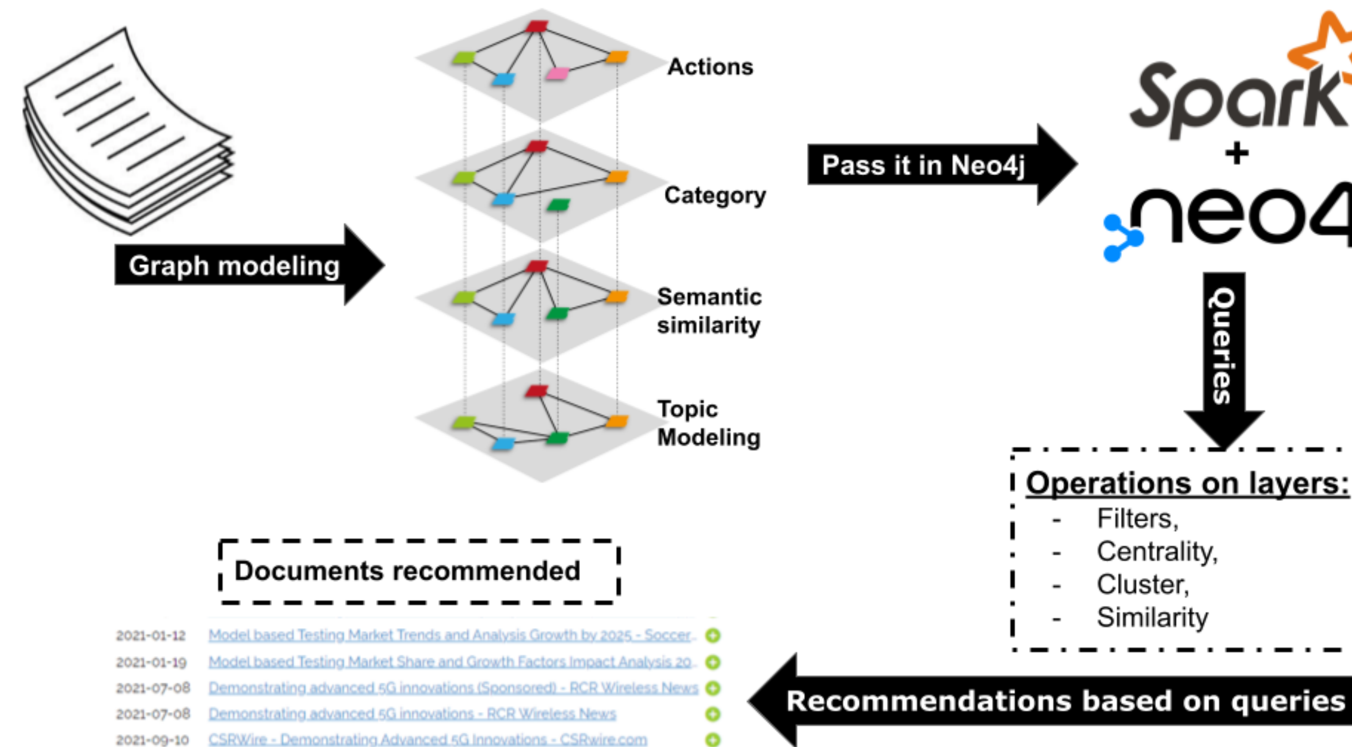
Fig. 1. Our multiplex framework for technology intelligence recommendation
