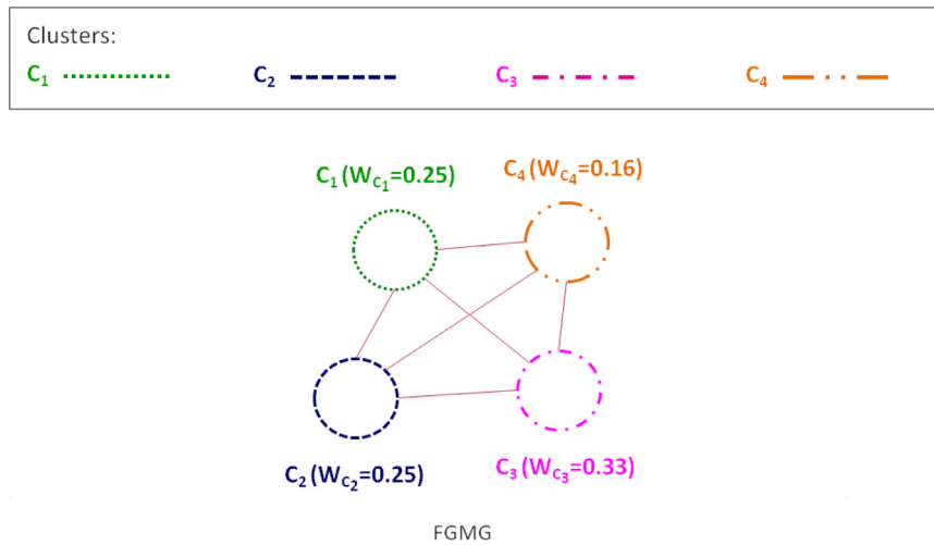
Fig. 21. The obtained FGGMG (the weight belonging to each cluster is given in parenthesis).
