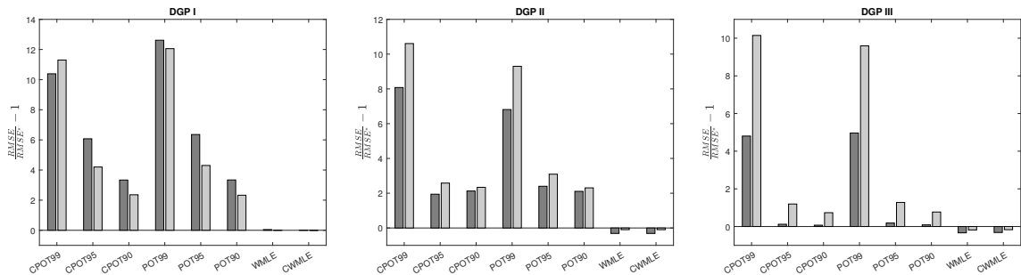
Figure 6: RMSE/RMSE^* - 1 for \hat{\beta}_0^\xi (dark grey) and \hat{\beta}_1^\xi (light grey), for DGP I to III.
