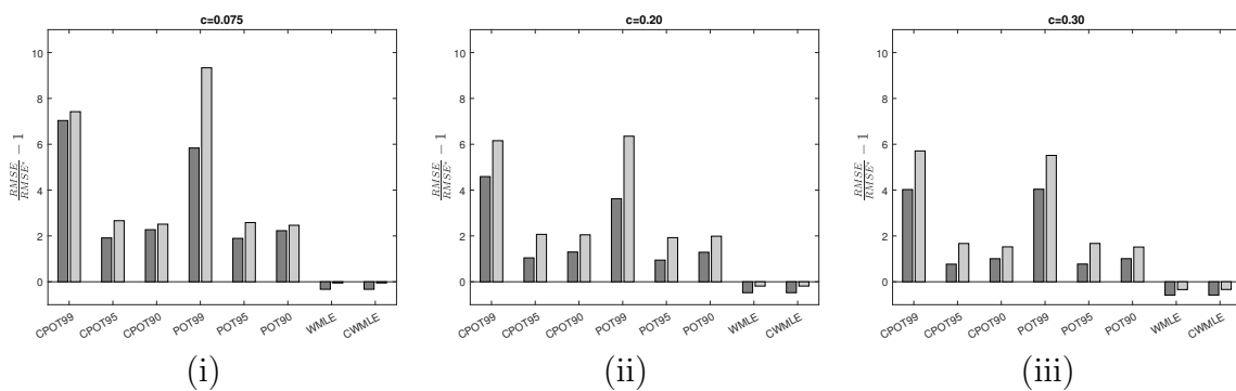
Figure 15: RMSE/RMSE^* - 1 for \hat{\beta}_0^\xi (dark grey) and \hat{\beta}_1^\xi (light grey), for the different contamination rates.
