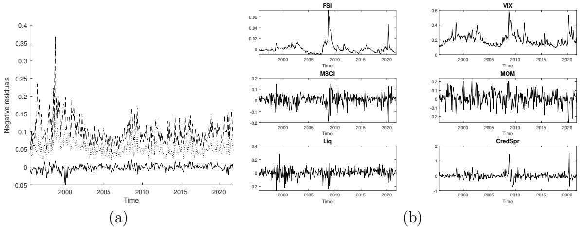
Figure 8: Panel (a): Mean (solid), 3 rd quartile (dotted) and 99% empirical quantile (dashed) of the cross-section of negative residuals \hat{y}_{ti} of Patton and Ramadorai (2013) model. Panel (b): Time series of the covariates.
