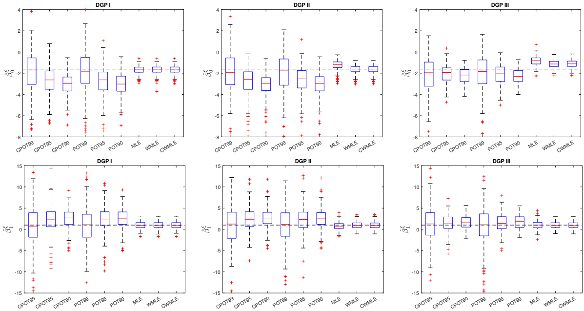
Figure 5: Estimated parameters \hat{\beta}_0^\xi (top) and \hat{\beta}_1^\xi (bottom) obtained with the proposed method and various POT approaches. Dashed: values of the true parameters. Columns CPOT99, CPOT95 and CPOT90 display the results obtained with the (conditional) POT approach, using quantile regression at the levels 99%, 95%, and 90% for the threshold. Columns POT99, POT95 and POT90 refer to the results of POT obtained with an unconditional empirical quantile at the same levels. Columns WMLE and CWMLE denote the results obtained with the censored likelihood procedure, using either a global censoring threshold, or a censoring threshold based on quantile regression. MLE relates to classical MLE. Details on the POT computations can be found in the Appendix.
