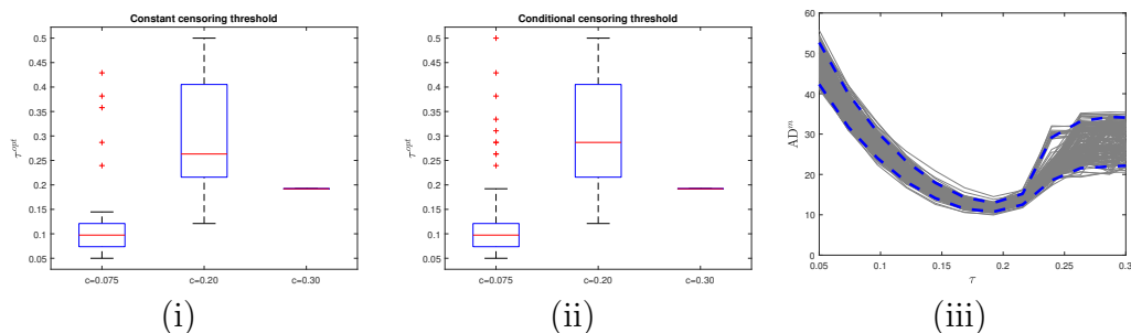
Figure 13: Selected censoring thresholds using either an unconditional quantile (panel (i)) or a conditional quantile (panel (ii)) in the weight function. Panel (iii): AD^m curves for c = 30\% . Blue: 5% and 95% empirical quantile of AD^m for fixed values of \tau .
