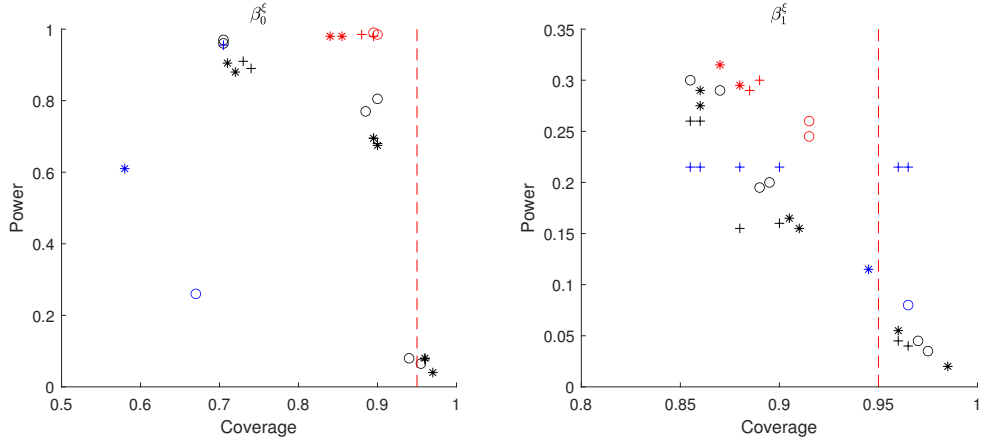
Figure 16: Power of rejecting the null hypothesis H_0 : \beta_j^\xi = 0 , for j = 0 (left) and j = 1 (right), as a function of the empirical coverage of a 95% confidence interval. Black: POT-based method. Blue: MLE. Red: (C)WMLE. +: c = 0.075 , *: c = 0.20 , o: c = 0.3 . Dashed red: nominal coverage of the confidence intervals.
