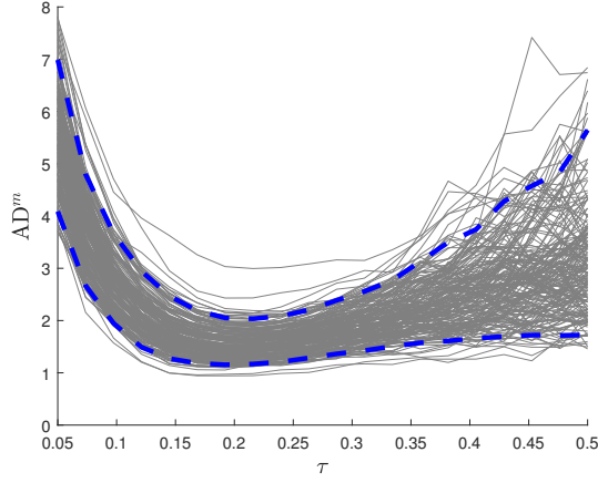
Figure 4: Representative AD^m statistics (grey), as functions of \tau and using conditional censoring thresholds q_{it}(\tau) , for DGP III. Dashed blue: 5% and 95% empirical quantiles of AD^m for a given \tau level, across simulated samples.
