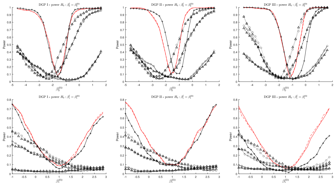
Figure 7: Power curves for the null hypotheses H_0 : \beta_0^\xi = \beta_0^{H_0} (top) and H_0 : \beta_1^\xi = \beta_1^{H_0} (bottom), for different values of \beta_0^{H_0} and \beta_1^{H_0} . From left to right: DGP I to DGP III. For \beta_0^{H_0} = \log(.2) and \beta_1^{H_0} = 1 , we expect a rejection rate equal to the 5% test level. Red solid and dashed: WMLE and CWMLE. +: MLE. \Delta : POT estimates based on unconditional thresholds. \circ : POT estimates based on conditional thresholds. Thresholds are taken as quantiles at the 99% (black solid), 95% (dashed dotted) and 90% (dotted) levels in the POT approaches.
