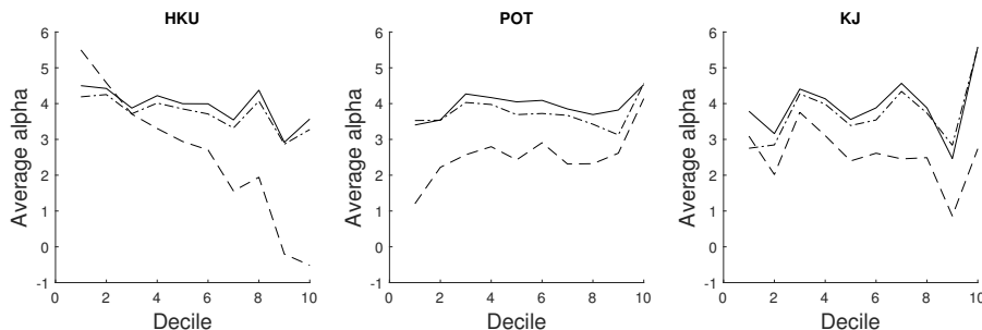
Figure 11: Average \hat{\alpha}_i^* for deciles of funds sorted on their \hat{\gamma}_i , obtained with the three different tail risk measures. Solid: CAPM alpha. Dashed-dotted: FH alpha. Dashed: JKKT alpha.
