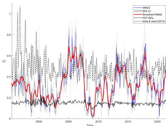
Figure 10: Time series of \hat{\xi}(\mathbf{x}_t) (solid blue). Red: smoothed estimate of WMLE obtained from a moving average filter. Shades of grey: 95% pointwise confidence intervals for \xi(\mathbf{x}_t) . Solid black: POT estimates with 95% empirical quantile as threshold. Dashed black: Hill estimator proposed by Kelly and Jiang (2014) with the monthly 95% empirical quantile as threshold.
