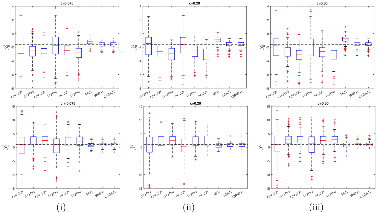
Figure 14: Estimated parameters \hat{\beta}_0^\xi (top row) and \hat{\beta}_1^\xi (bottom row) obtained with the G-E-GPD method and with various POT approaches for DGP I to DGP III (from left to right). Dashed: values of the true parameters.
