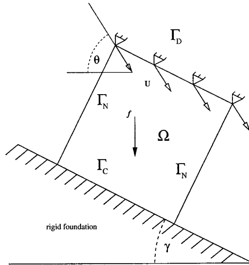
Figure 7. An example of mechanical problem (1)–(4) with non-uniqueness. An elastic square lying on a rigid inclined plane, loaded by the gravity f and by an imposed displacement \mathbf{U} .
