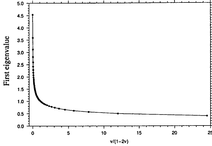
Figure 6. The dependence of the first eigenvalue on the ratio \eta = v/(1 - 2v) .
