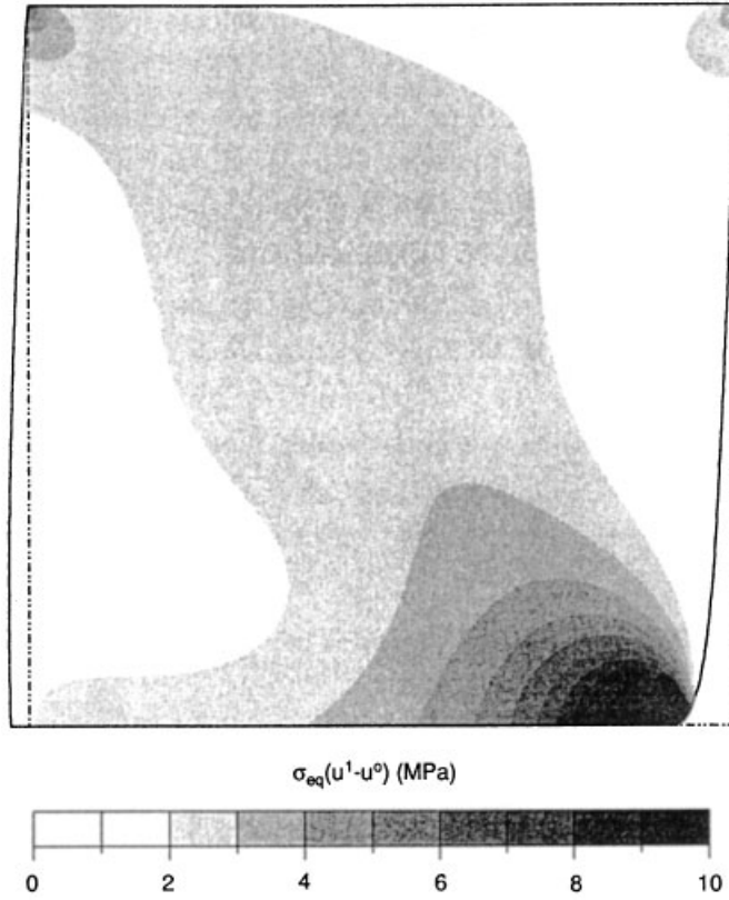
Figure 11. The Von-Mises stress corresponding to the difference u_h^1 - u_h^0 .
